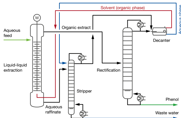
Process flow diagram of phenol recovery process
